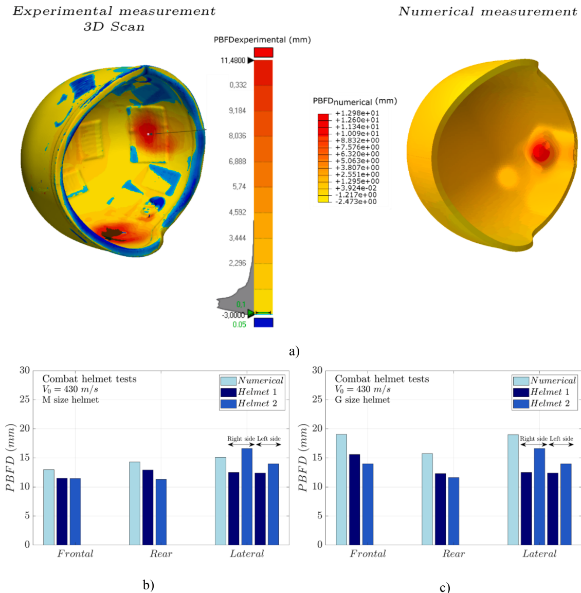
Fig. 9. (a) Experimental and numerical PBFD measurement method. Comparison of PBFD between experimental and numerical results for (b) M-size helmet and (c) G-size helmet. Note that shots are conducted on both sides of the helmets.
