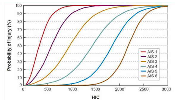
Fig. 11. According to the AIS scale, head injury risk curves are based on the HIC. Data from Hayes et al. [53].
