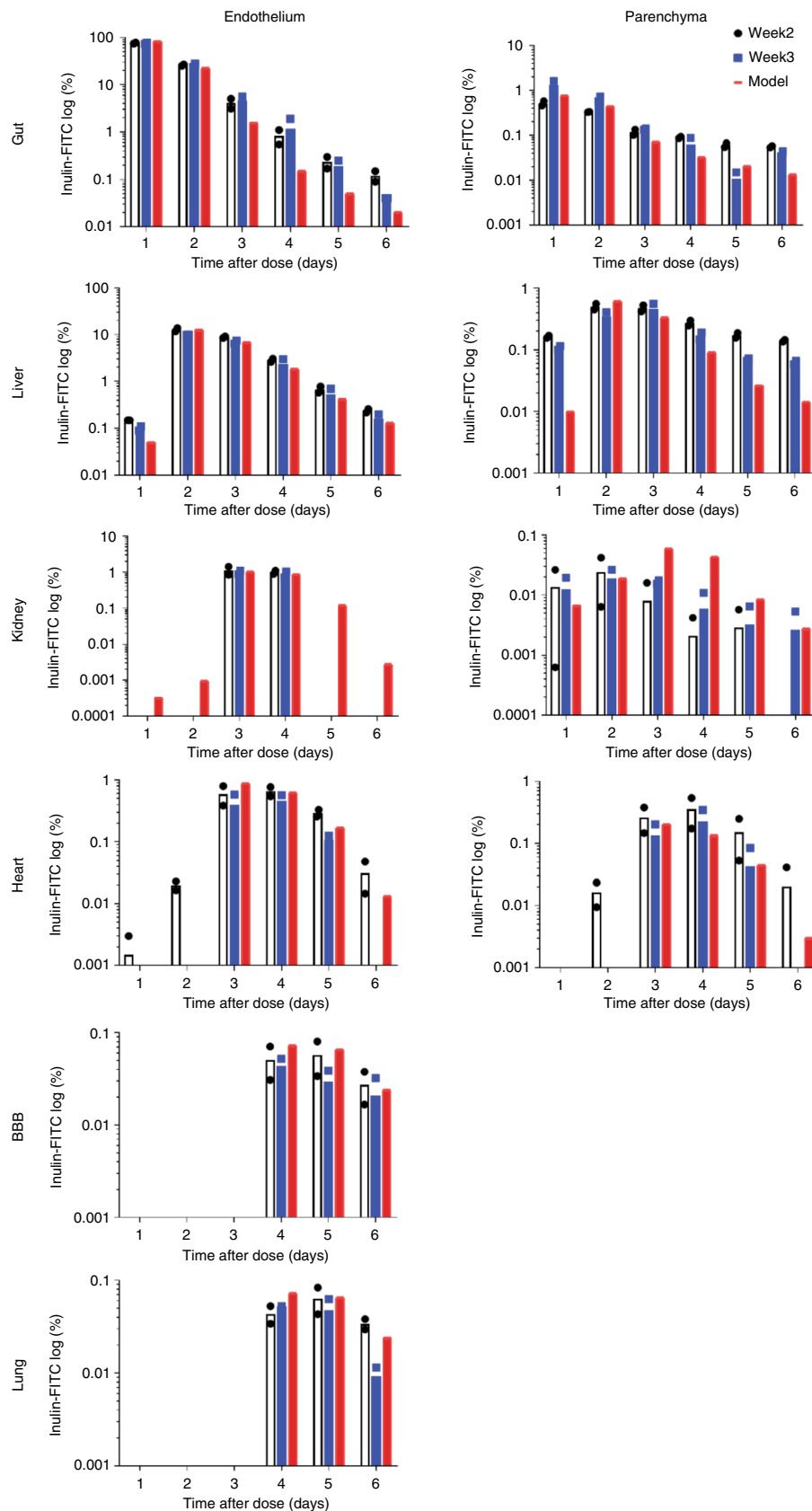
Fig. 5 | Long-term analysis of inulin-FITC PK in an eight organ system linked via vasculature and supported by computational PBPK modelling.
